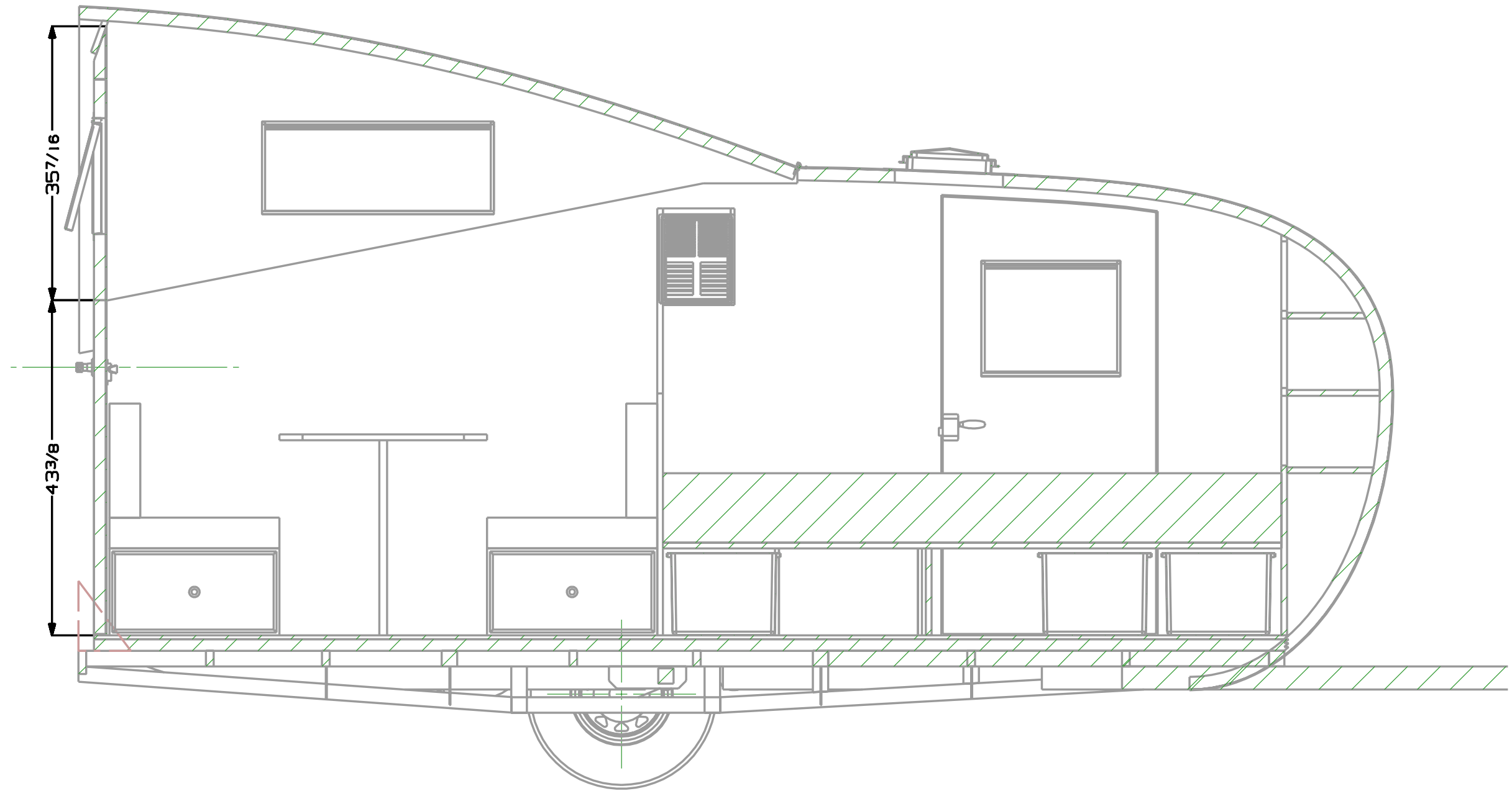
14' OPTIMIZED WINTER WARRIOR - SECTION VIEW LOOKING TOWARDS STREET SIDE
