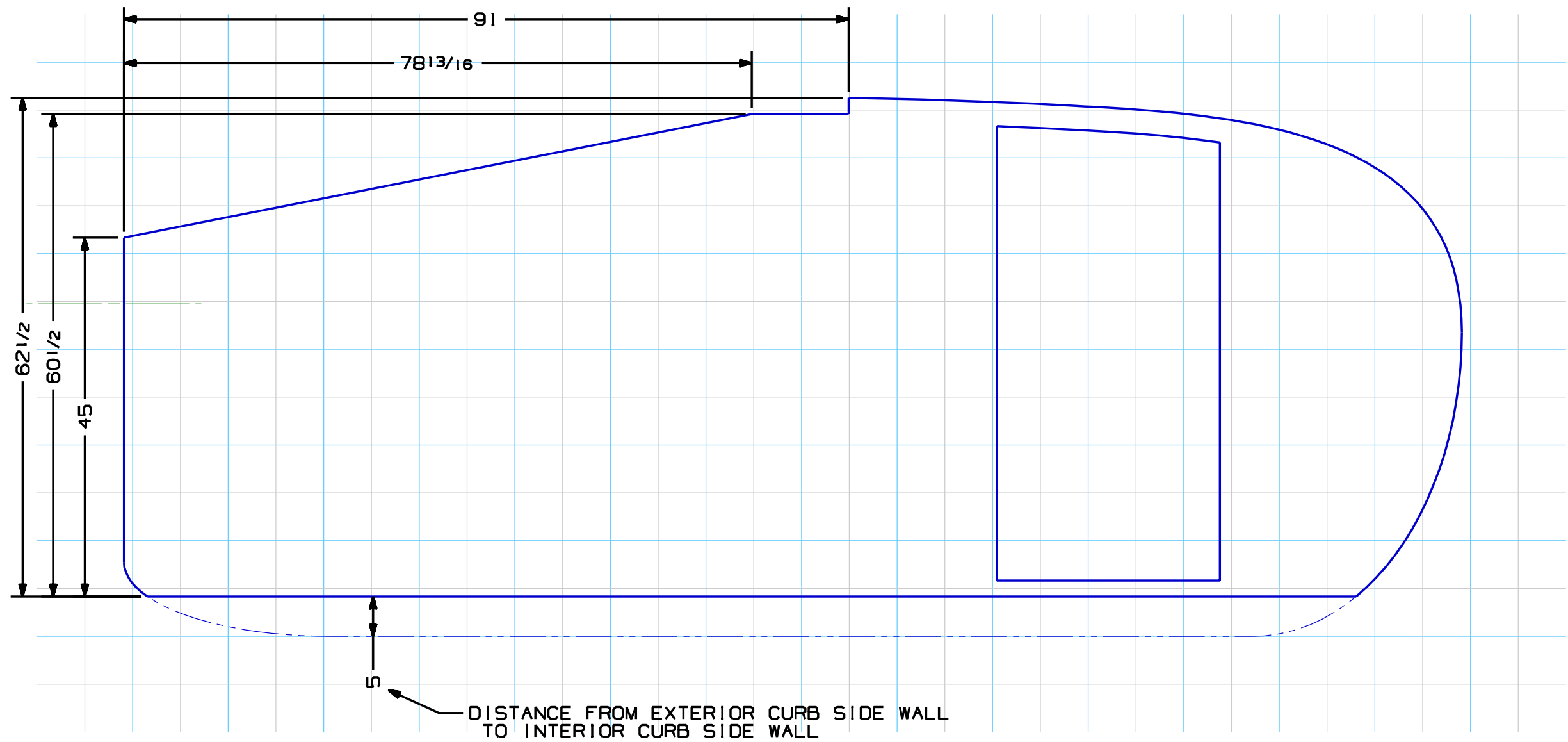
14' OPTIMIZED WINTER WARRIOR - INTERIOR CURB SIDE WALL (FIXED)
