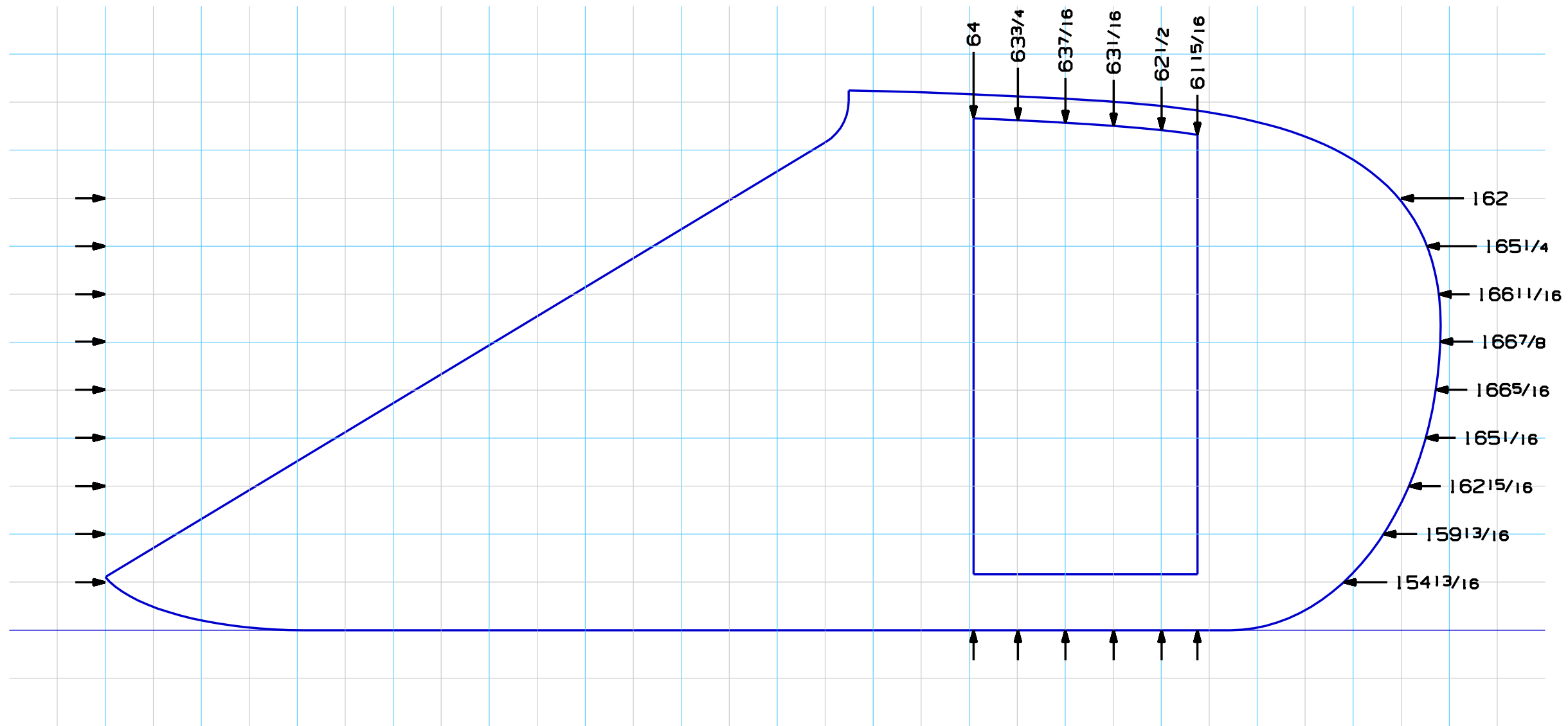
14' OPTIMIZED WINTER WARRIOR - EXTERIOR CURB SIDE WALL (FIXED)
