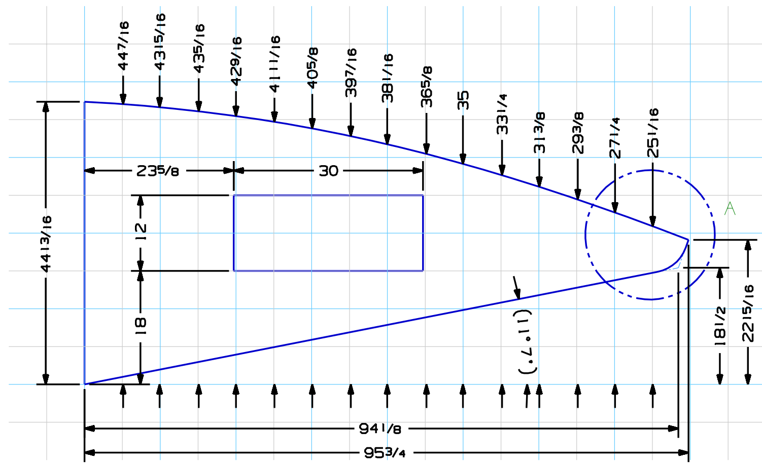
14' OPTIMIZED WINTER WARRIOR - HATCH SIDE (MOVABLE)
