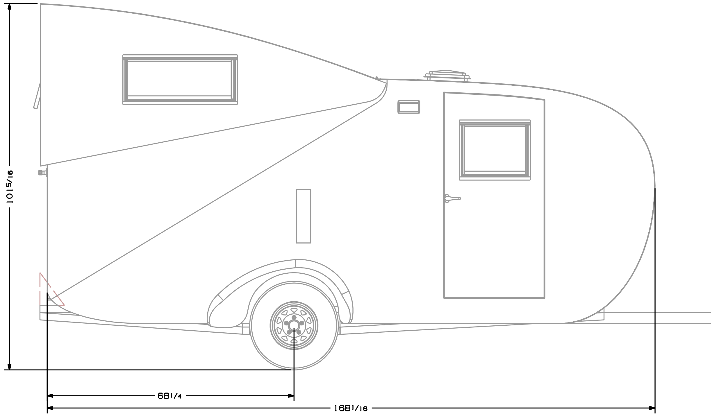
14' OPTIMIZED WINTER WARRIOR - SIDE VIEW - HATCH UP
