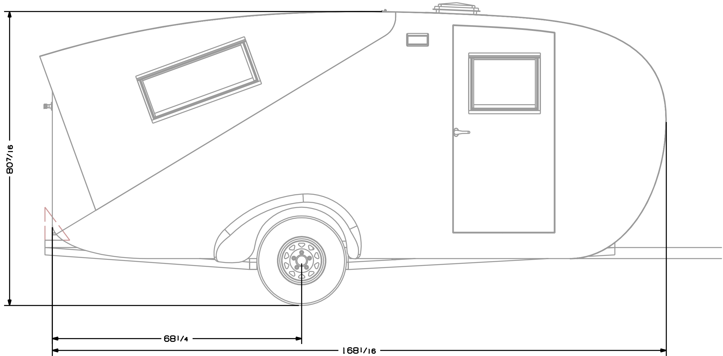
14' OPTIMIZED WINTER WARRIOR - SIDE VIEW - HATCH DOWN
